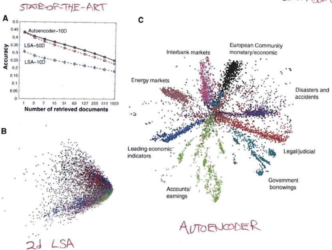
Fig. 4. (A) The fraction of retrieved documents in the same class as the query when a query document from the test set is used to retrieve other test set documents, averaged over all 402,207 possible queries. (B) The codes produced by two-dimensional LSA. (C) The codes produced by a 2000-500-250-125-2 autoencoder.
