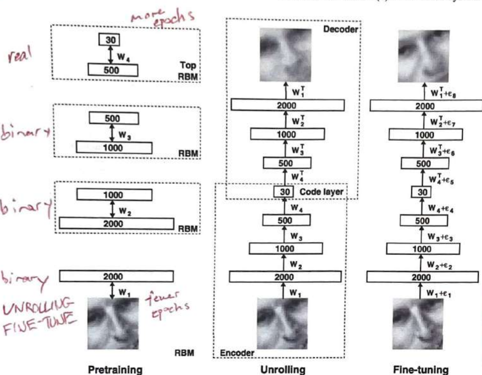
Fig. 1. Pretraining consists of learning a stack of restricted Boltzmann machines (RBMs), each having only one layer of feature detectors. The learned feature activations of one RBM are used as the "data" for training the next RBM in the stack. After the pretraining, the RBMs are "unrolled" to create a deep autoencoder, which is then fine-tuned using backpropagation of error derivatives.
